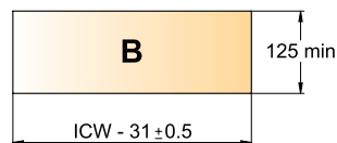
Back panel
