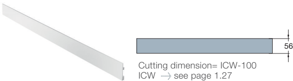
Front Panel
