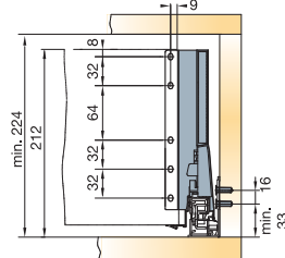
Tekform Drawer DW182
