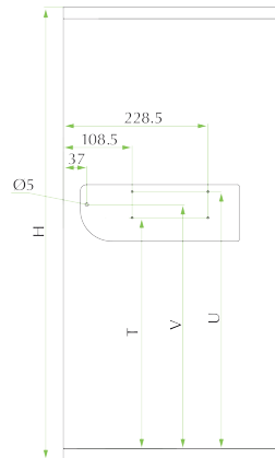
Cabinet Fixing
