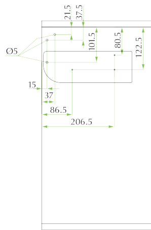
Cabinet Fixing
