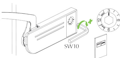
Weight Adjustment
