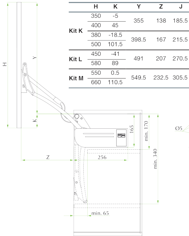
Cabinet Fixing
