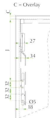
Door Fixing
