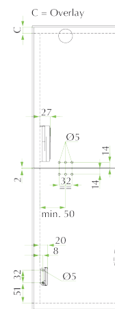
Door Fixing
