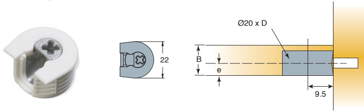
Technical and mounting details
