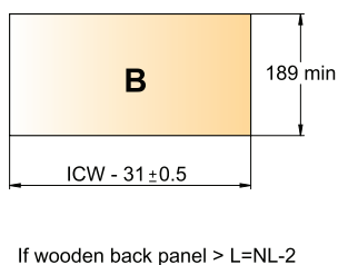
Back panel
